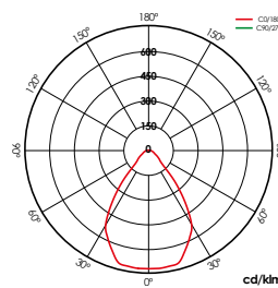
Empotrar S069L0P Embed S069L0P Empotrate S069L0P Empotrate S069L0P
