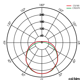
2x10W 600mm
